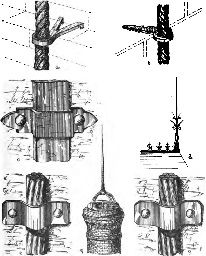
Fig. 2. Conductors and fastenings. From Anderson, and Lightning Rod Conference Report.
